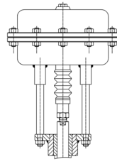
Pneumatic actuator
