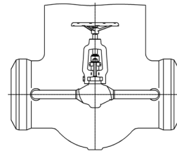
With by-pass
