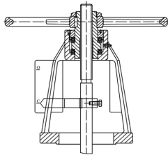
Position indicator
