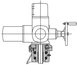
Electric actuator
