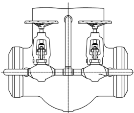
With equalizing pipe and by-pass
