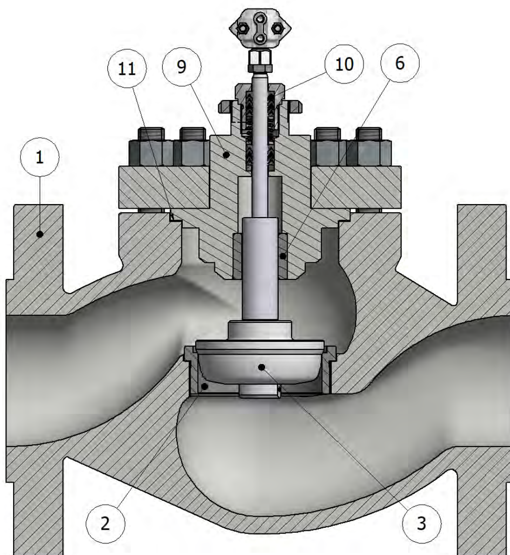
STANDARD VALVE
