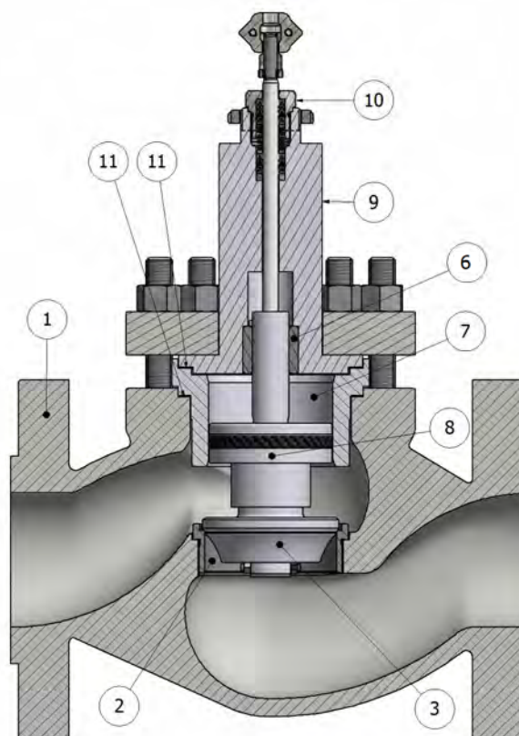
BALANCED TRIM VALVE WITH EXTENDED BONNET
