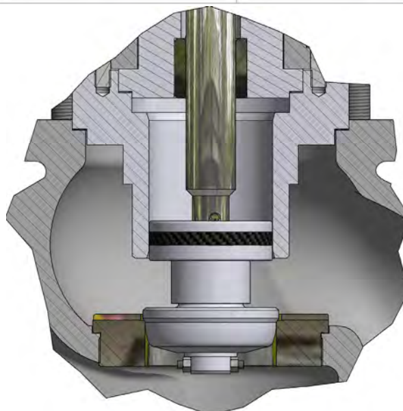
BALANCED TRIM
